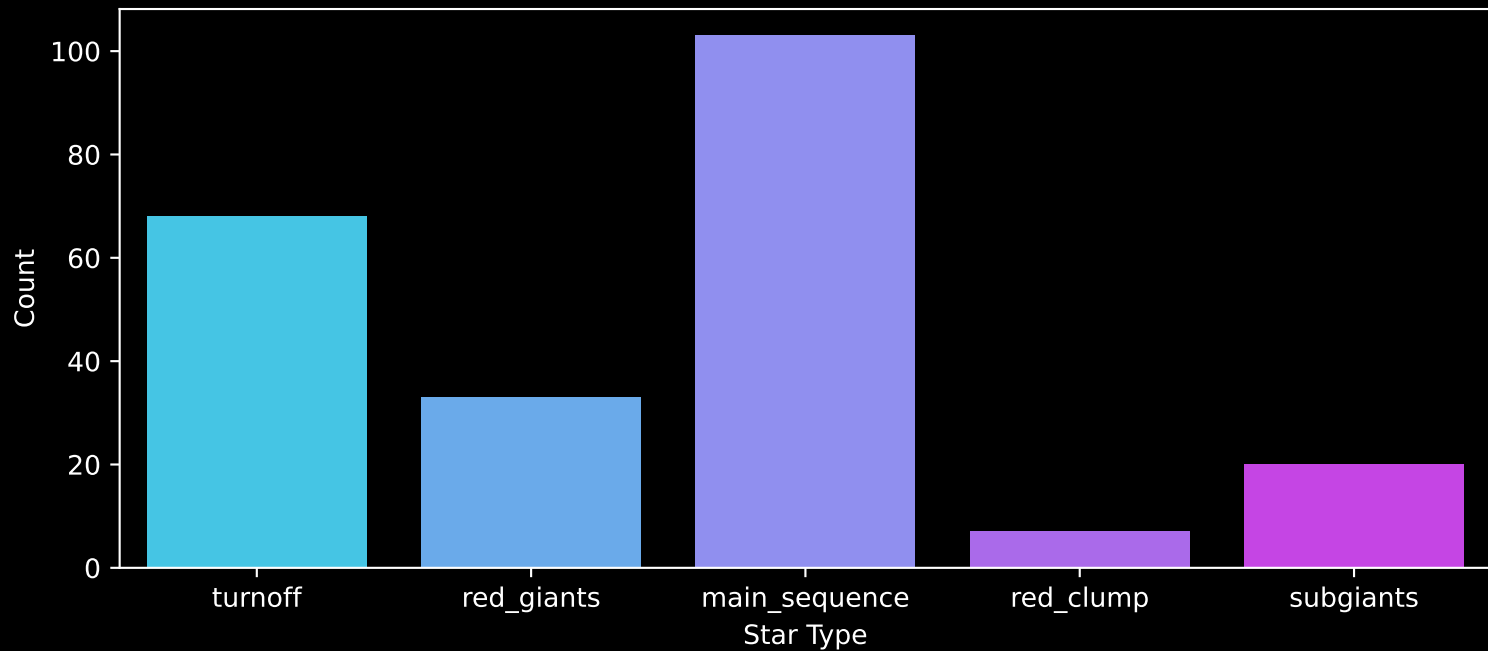
GALAH DR4 Field: [727] Count plot of Star Type
