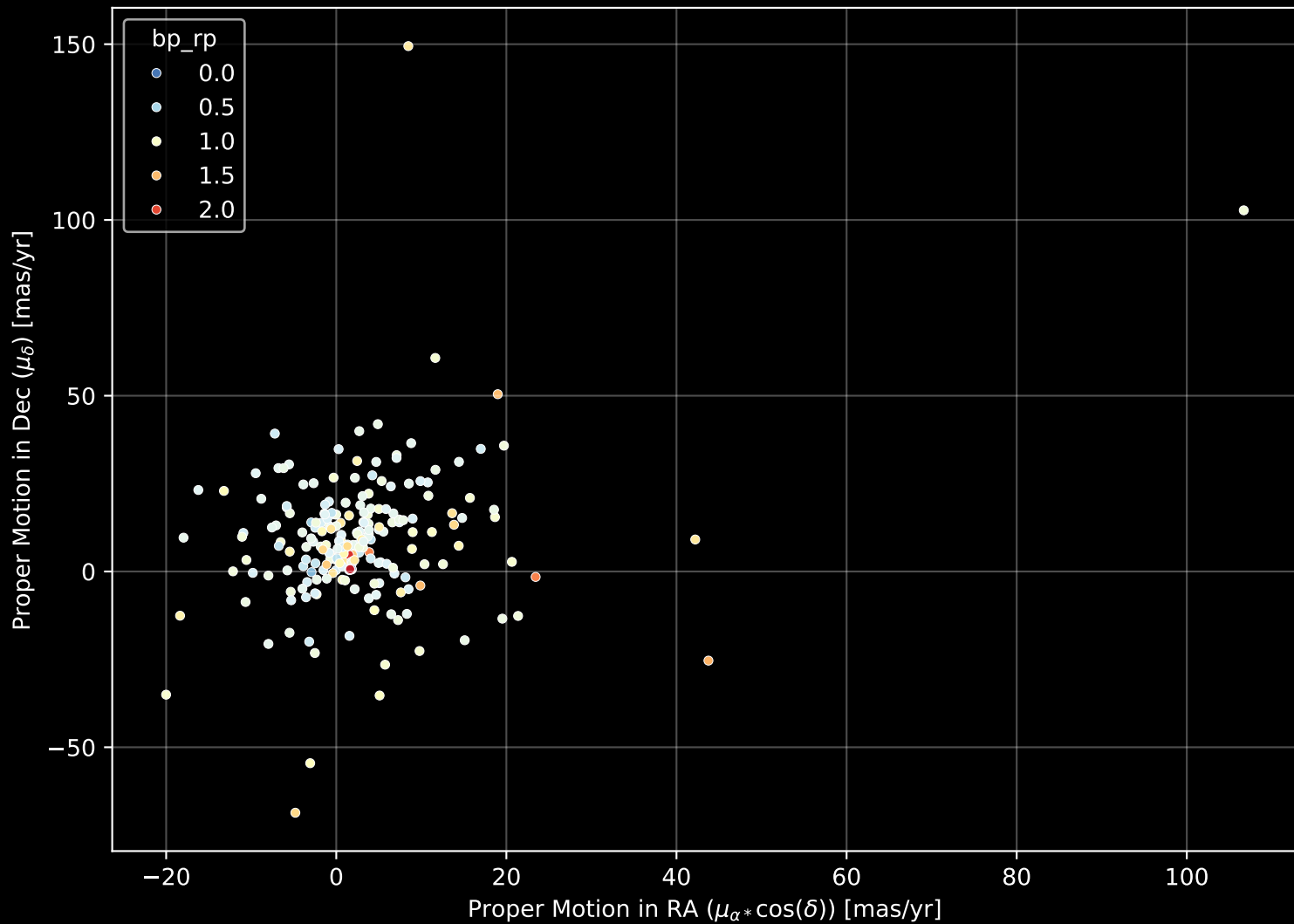
GALAH DR4 Field: [727] Proper Motion Diagram (n= 231)
