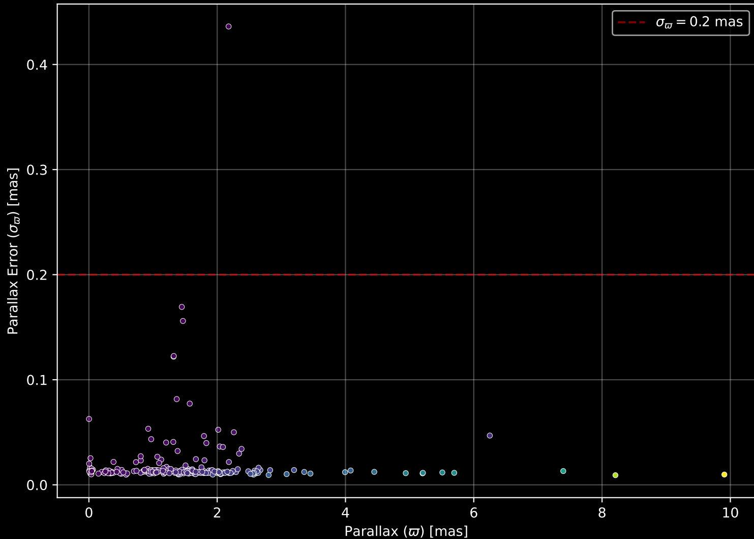
GALAH DR4 Field: [727] Parallax Quality (n= 231)
