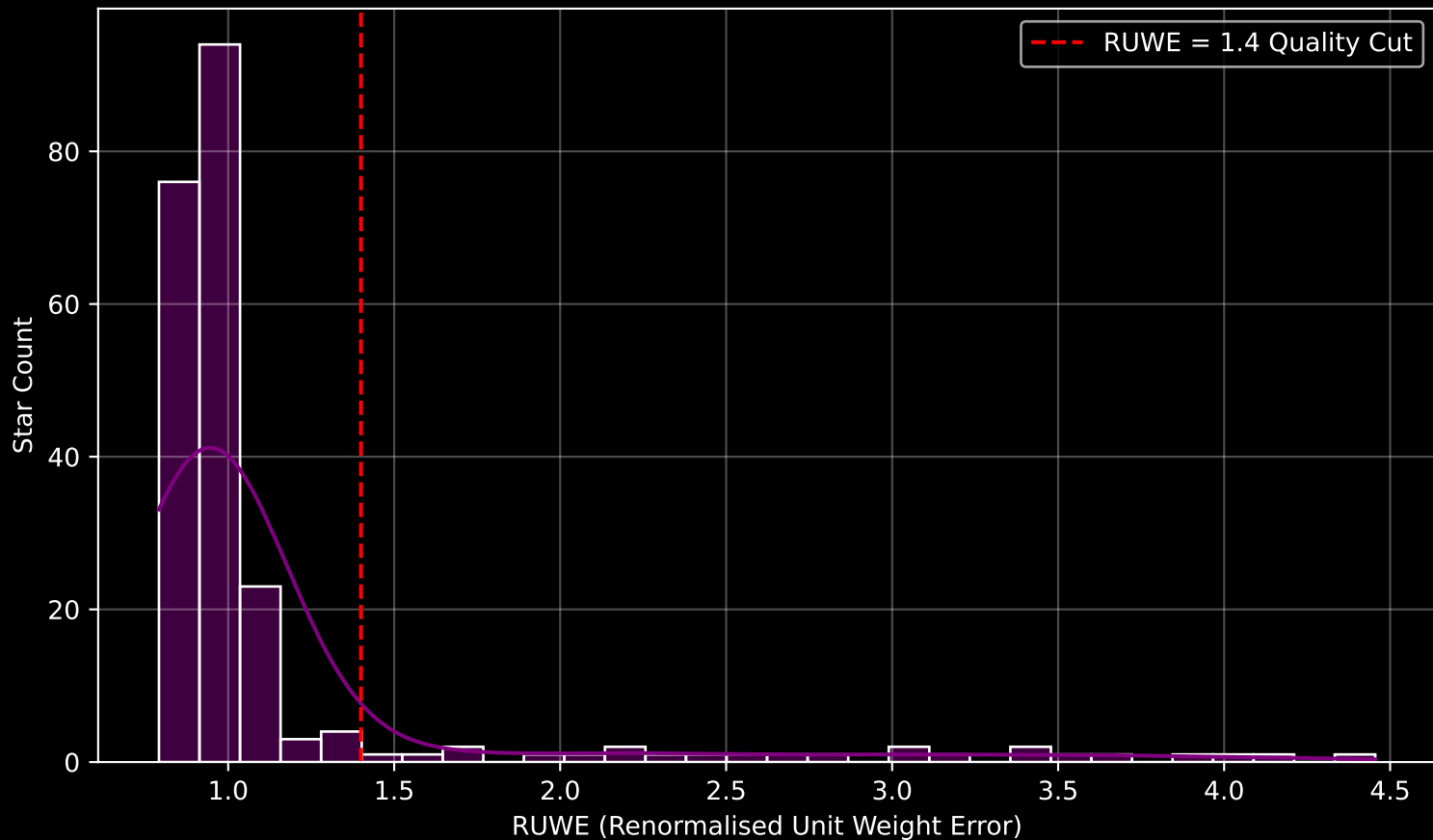
GALAH DR4 Field [727] RUWE Distribution (n= 224)
