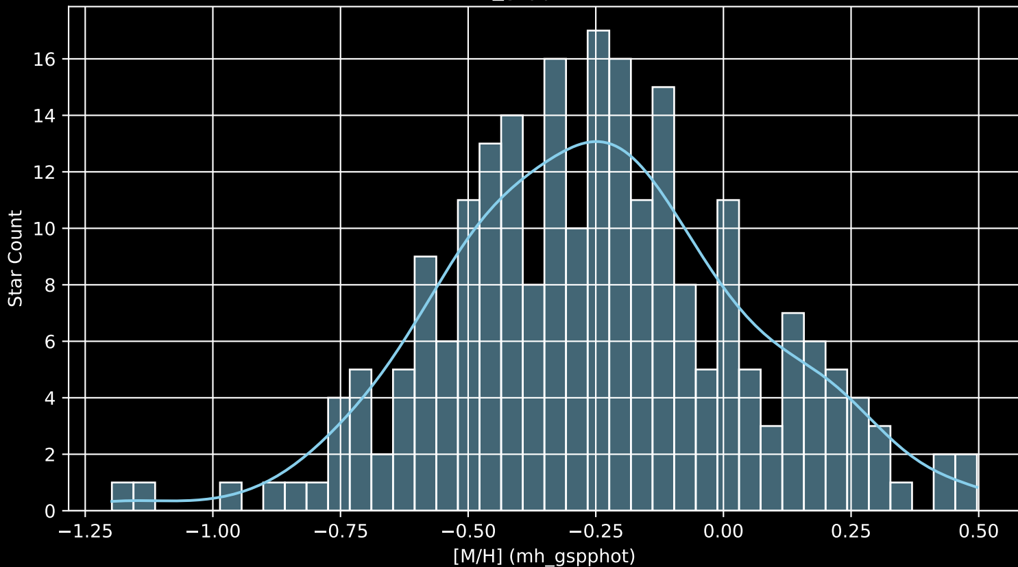
GALAH DR4 Field: [727] [M/H] (mh_gspphot) (n= 230)
